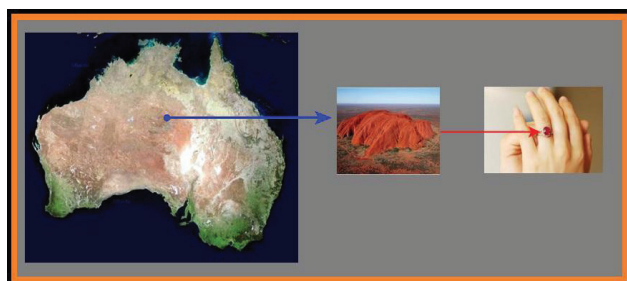
Figure 4 The celestial body ring-the ayers rock that is located at the geometrical centre of the main island of Australia.
