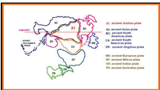
Figure 11 The jigsaw recovery of the unique supercontinent of the earth 66 million years ago.
