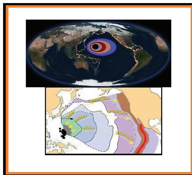
Figure 5 The geological age distribution of clam shells [12] and the Hinted Black Hole (HBH) of the northwestern Pacific ocean floor.
