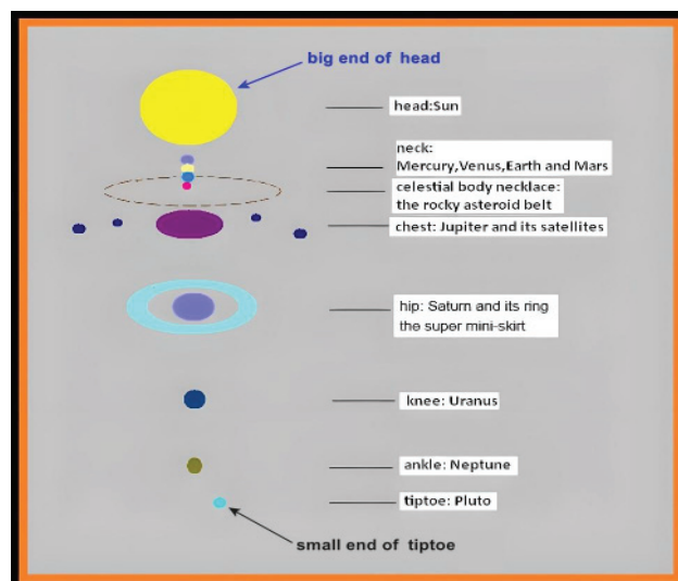
Figure 2 The evolution sequence of the humanoid solar system implied from the big end of head (the sun) to the small end of tiptoe of the foot (the pluto).
