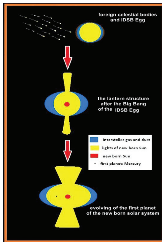
Figure 1 The big bang of the interstellar dirty snow ball egg from which the humanoid solar system originated.
