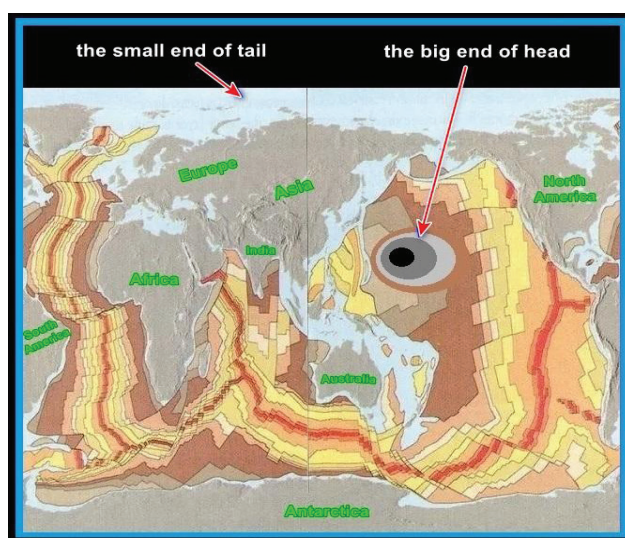
Figure 6 The evolution sequence from the big end of head of the northwestern Pacific ocean floor to the small end of tail of the Arctic ocean floor of the mid-oceanic ridge of the earth [15].
