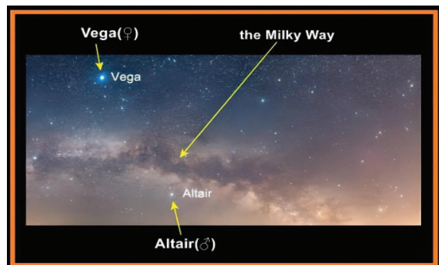
Figure 12 The legend story of the celestial bodies' love between the Vega (♀) and Altair (♂) across the milky way.
