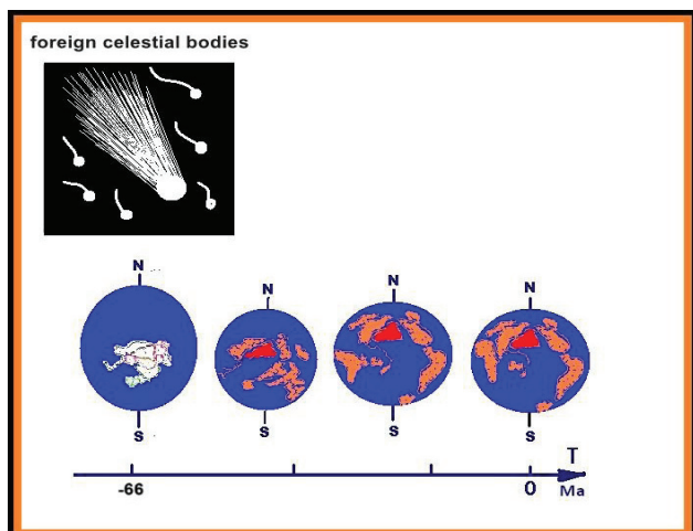
Figure 3 Broke up of the unique supercontinent 66 ma ago from which the mid-oceanic ridge of the earth originated.
